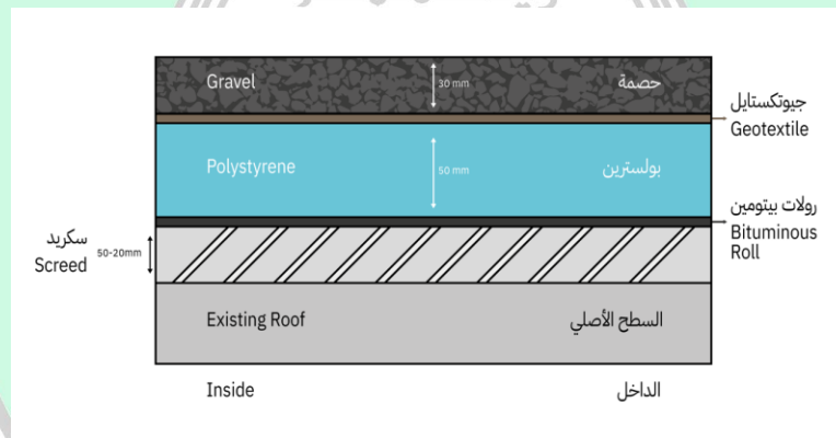
Figure 4 Thermal insulation layers implemented on the rooftops.
