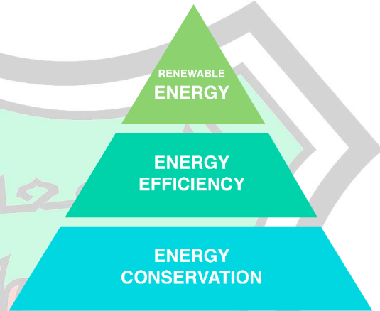
Figure 2 Energy pyramid.
